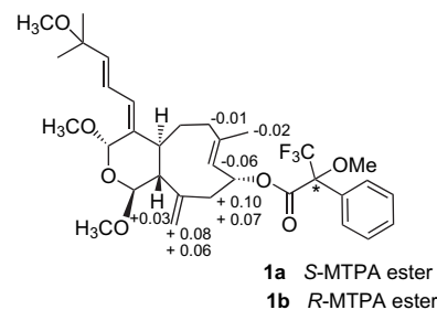
Figure 6. Application of the modified Mosher's method for secondary alcohols on the MTPA esters of xenimanadin A ( 1a and 1b ). \Delta\delta ( \delta_S - \delta_R ) are given in parts per million.
