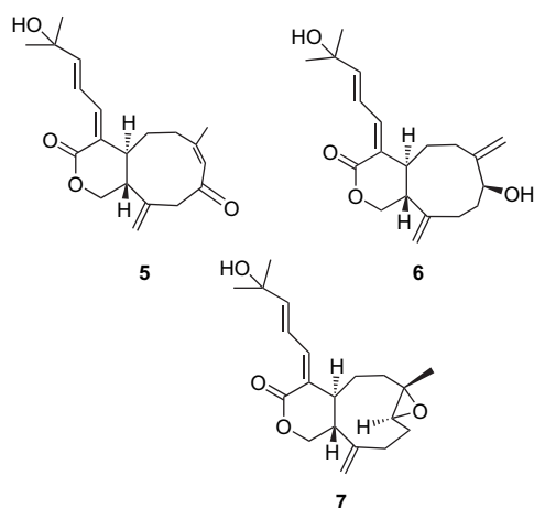
Figure 3. The known blumiolide C (5), xenioliide F (6), and deoxyoxidoisoxenioliide A (7).
