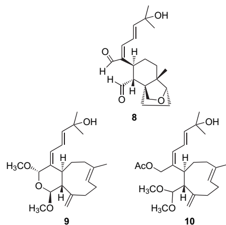
Figure 7. A rearranged xenicane dialdehyde derivative (8) and two known methoxylated xenicanes (9 and 10).
