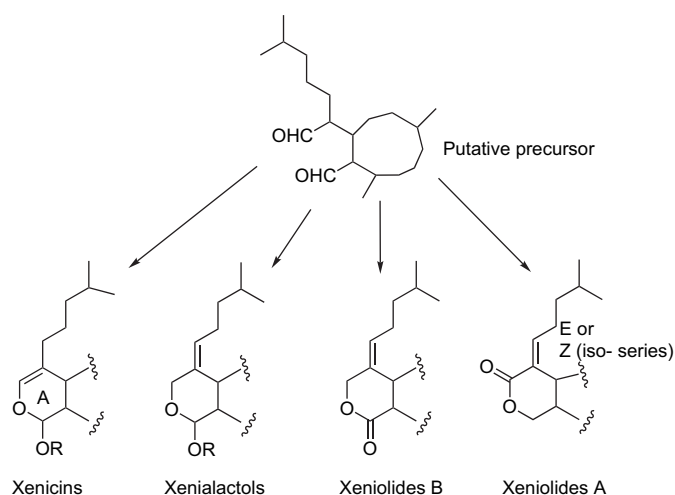
Figure 1. The four classes of pyran-cyclononane xenicane diterpenoids and their postulated precursor.
