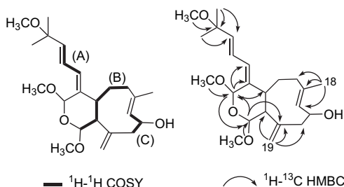
Figure 4. COSY and ^{2,3}J H \rightarrow C HMBC correlations of xenimanadin A ( 1 ).
